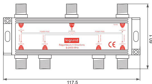
6-output distribution block = 117.5 x 60.1 x 17.4
