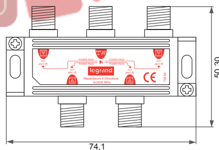
4-output distribution block = 74.1 x 50.30 x 16.6
